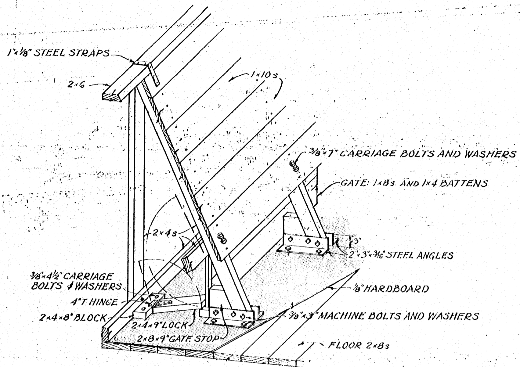
ISOMETRIC OF GATE STOP AND LOCK
