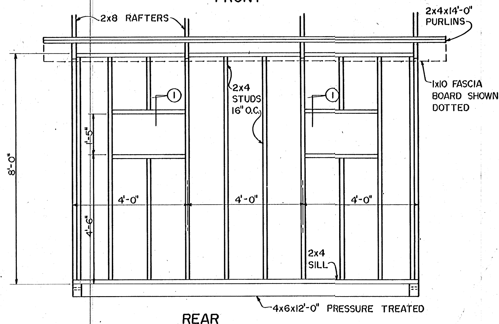
FRONT
