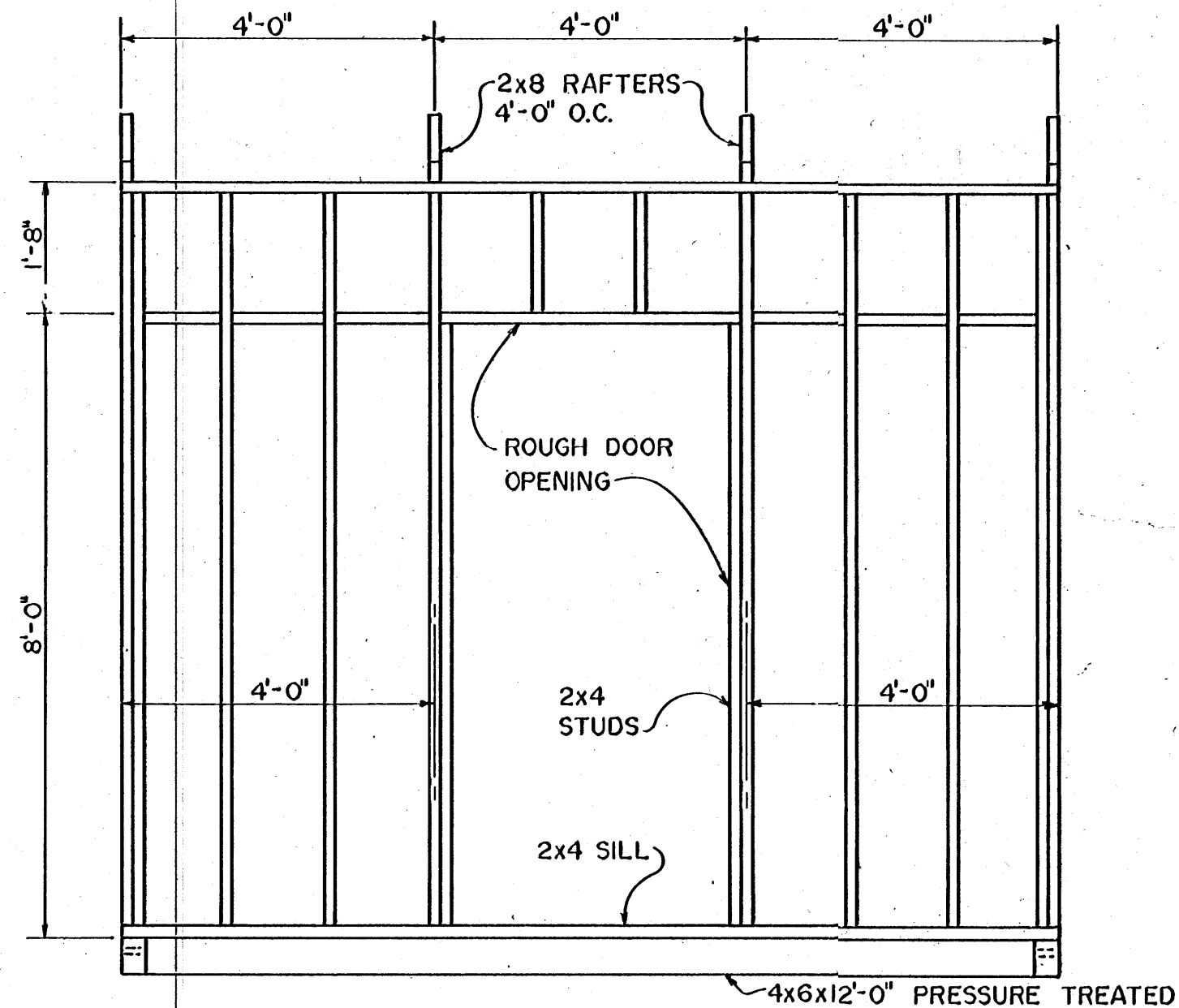
FRONT
