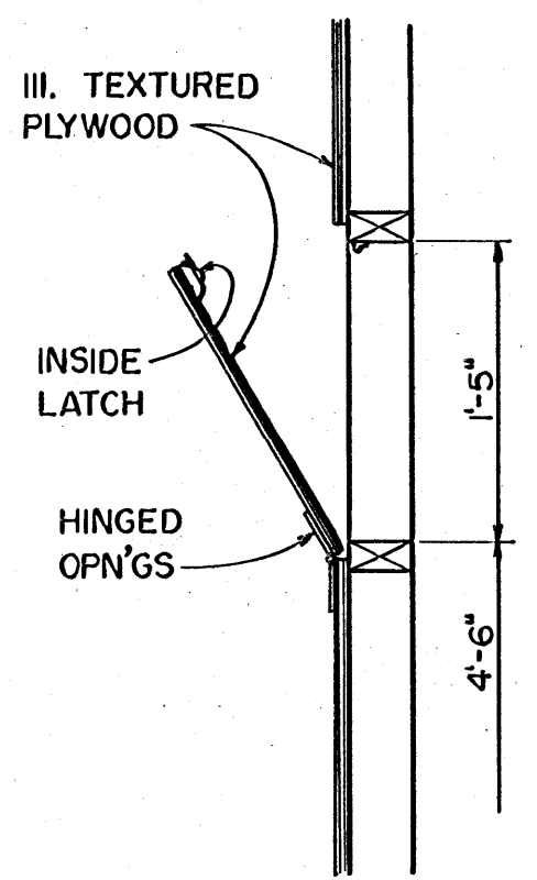
① DETAIL OF TWO OPN'GS AT REAR
