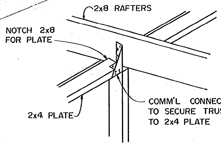
② DETAIL
