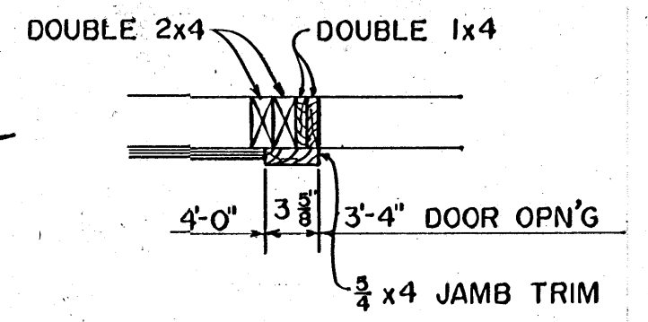
④ SECTION AT DOOR
