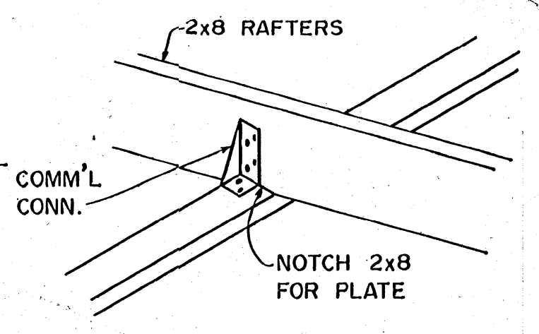
③ DETAIL
