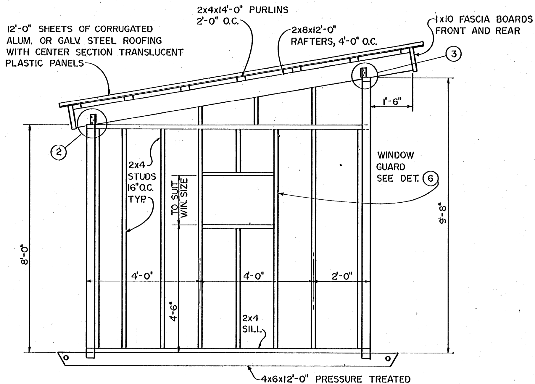
SIDES
