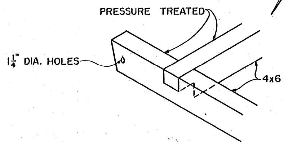
⑦ DETAIL
