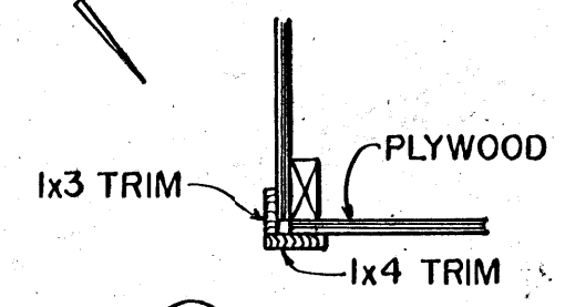
⑤ DETAIL
