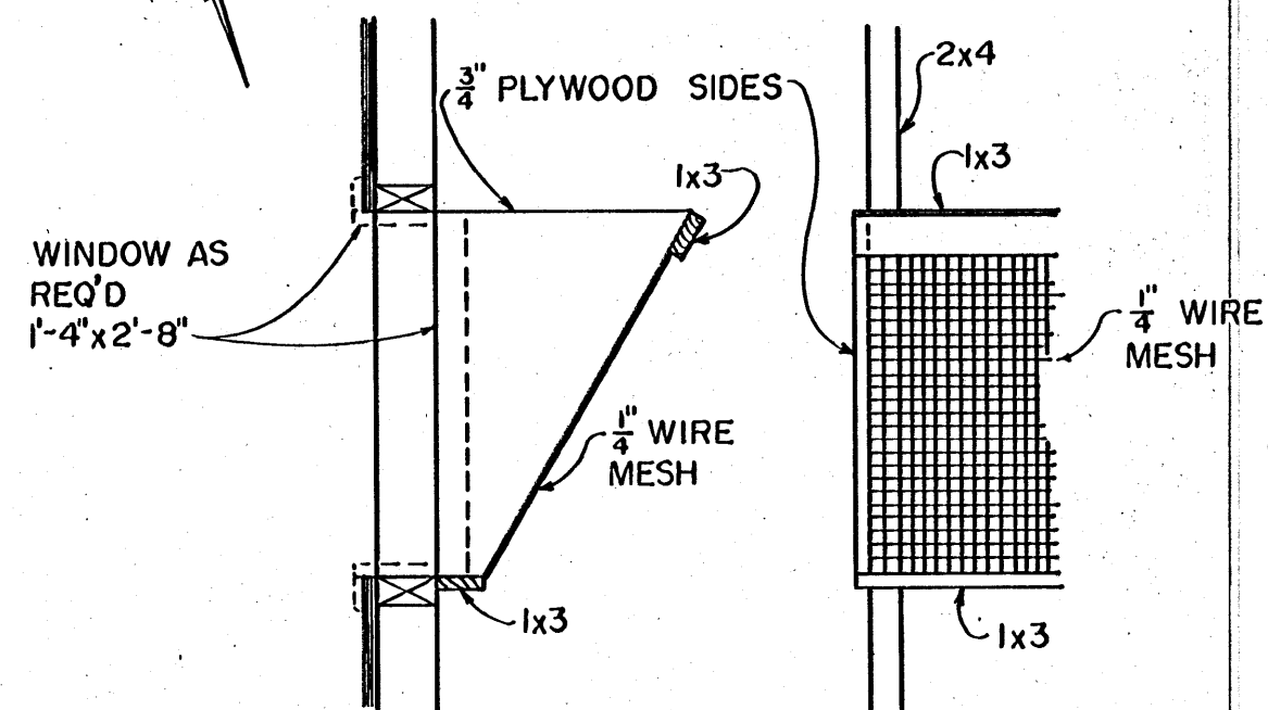
⑥ WINDOW GUARD SECTION
