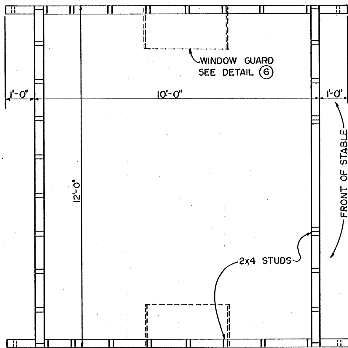
PLAN
