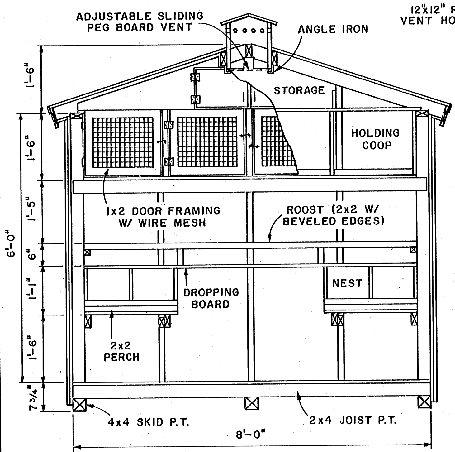
SECTIONS OF CHICKEN HOUSE-BANTAMS
