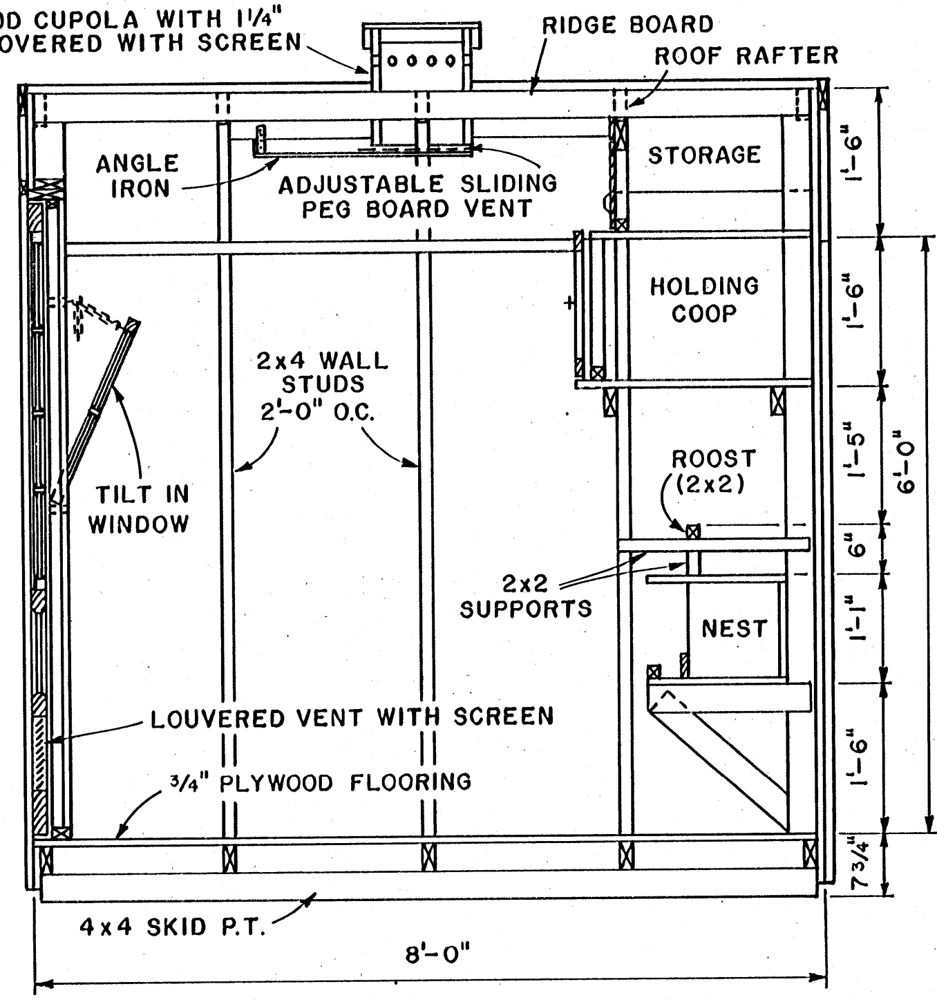
SECTIONS OF CHICKEN HOUSE-BANTAMS
