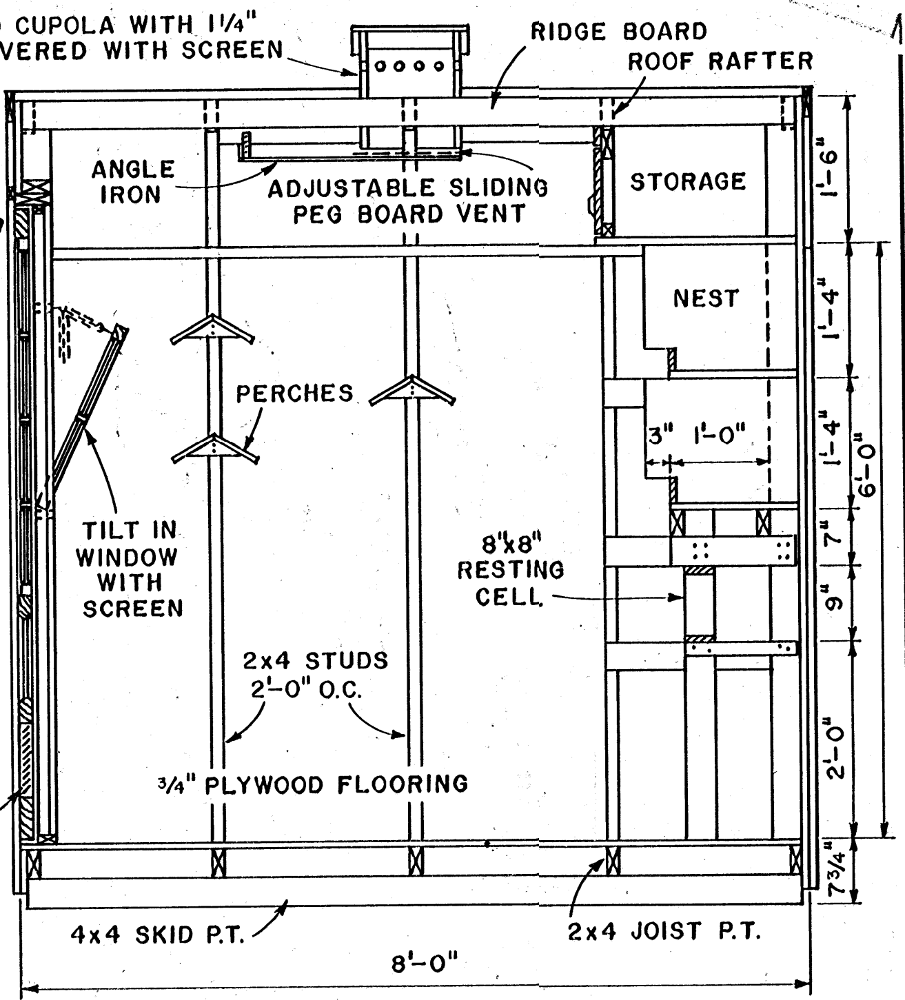
SECTION OF PIGEON HOUSE
