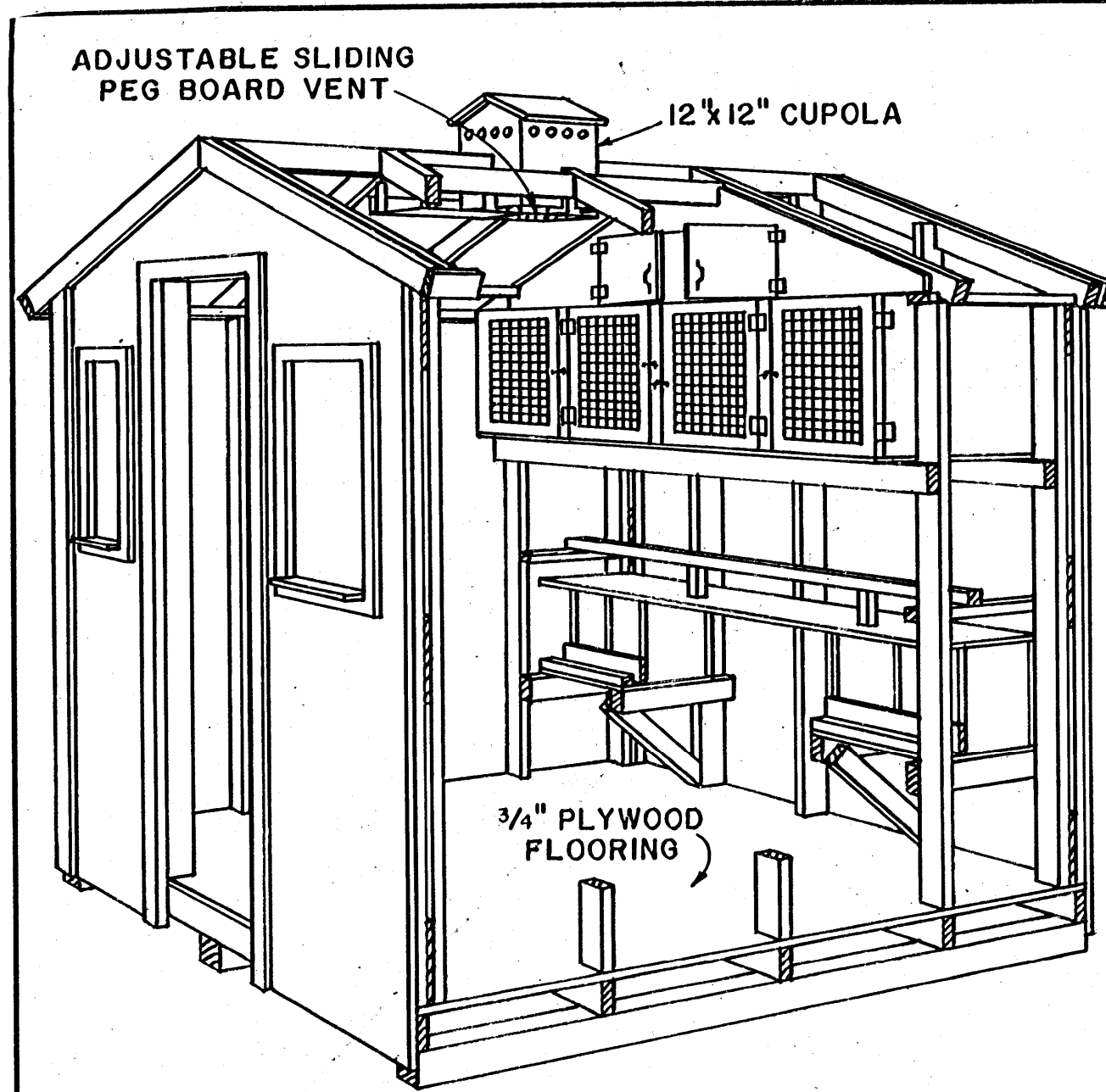
PERSPECTIVE OF CHICKEN HOUSE-BANTAMS
