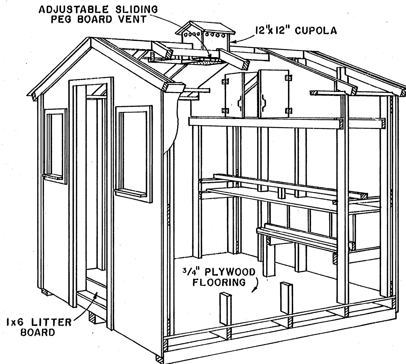
CUTAWAY VIEW OF 8'x8' LAYING HOUSE
