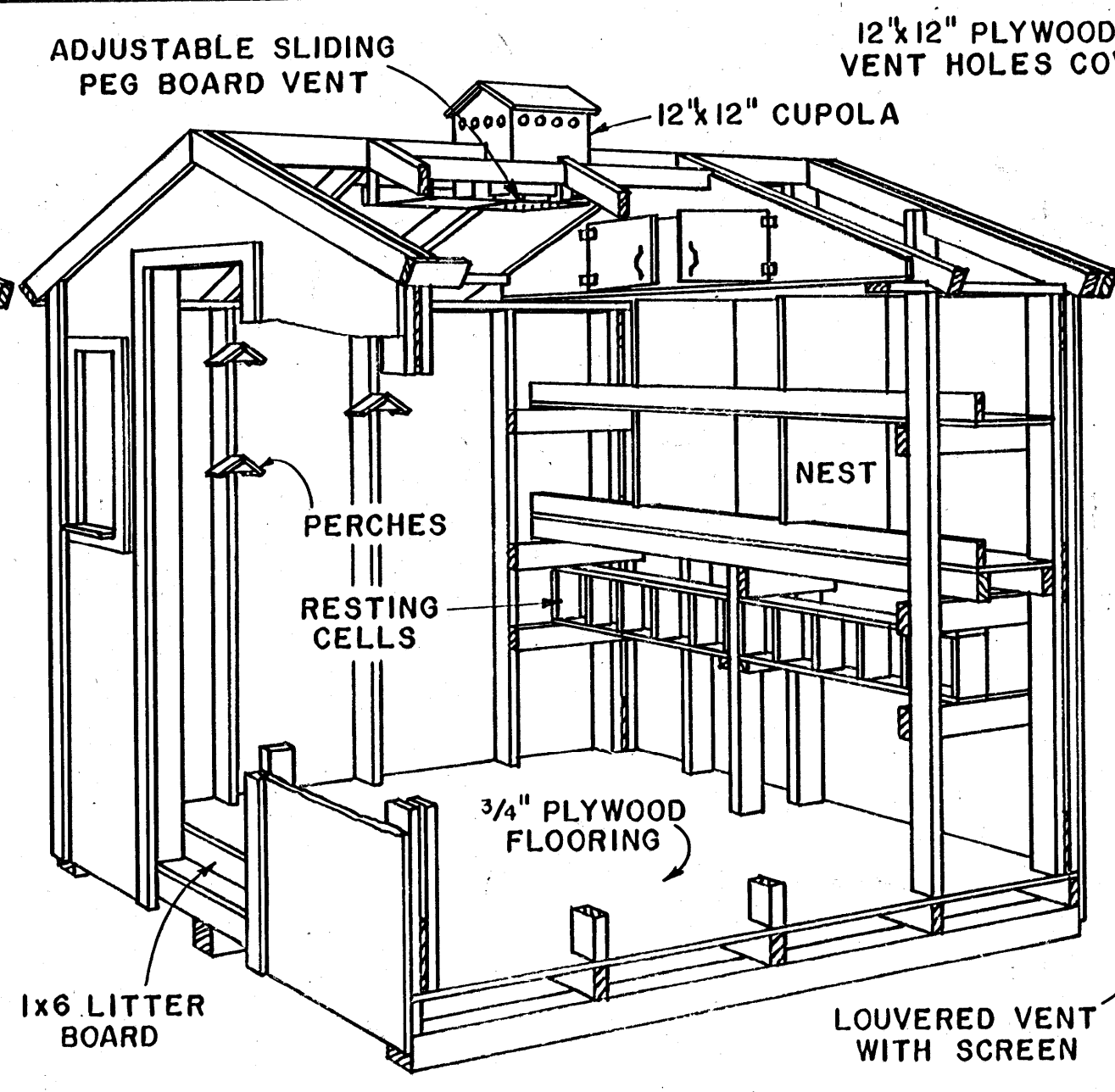
PERSPECTIVE OF PIGEON HOUSE
