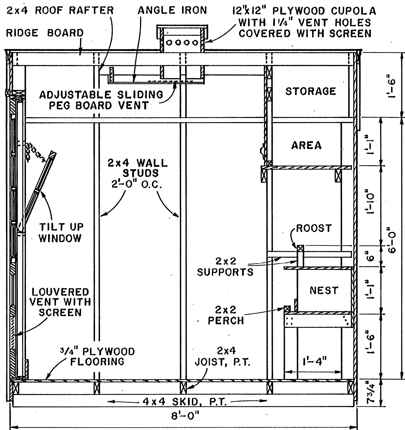
SECTION LAYING HOUSE
