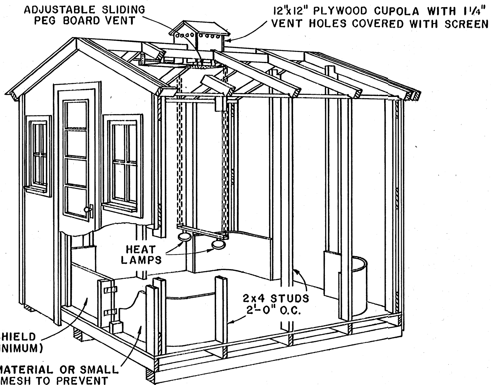
CUTAWAY VIEW OF 8'x8' BROODER HOUSE
