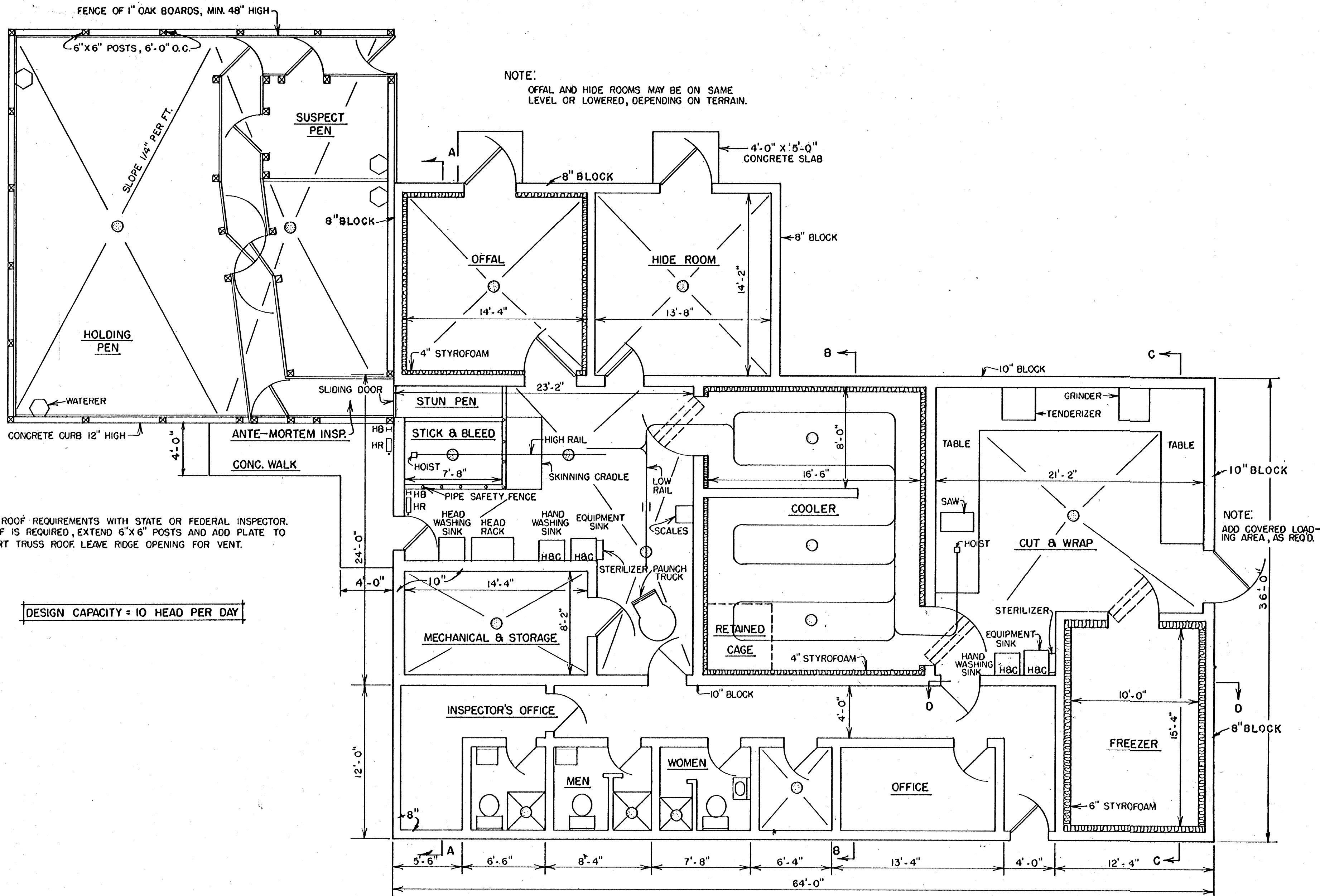
FLOOR PLAN SCALE: 3/16" = 1'-0" 12" 0' 1' 2' 3' 4'
