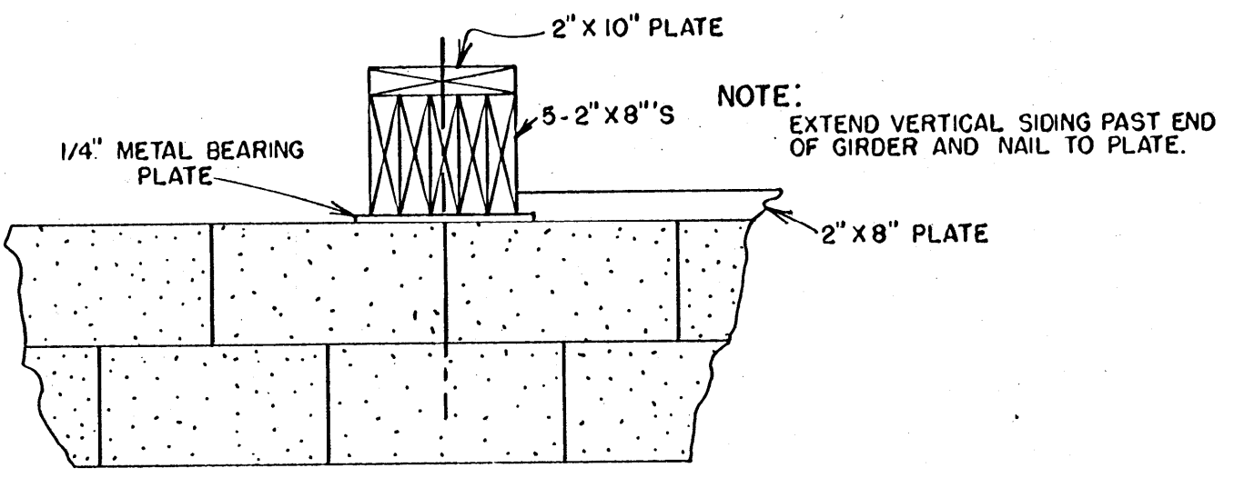
DETAIL OF OUTSIDE END OF GIRDER
