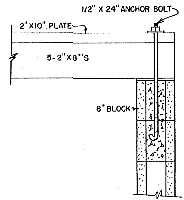
DETAIL OF INSIDE END OF GIRDER
