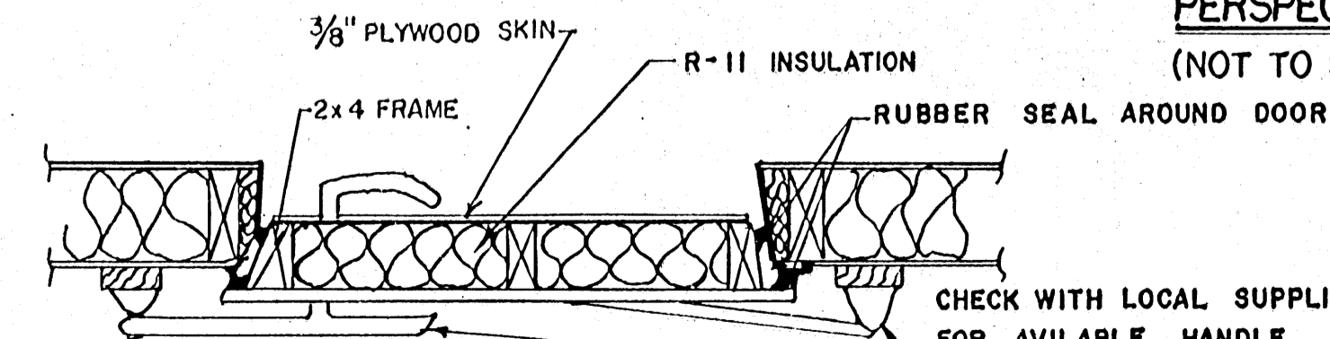
ALTERNATIVE DOOR DETAILS (NOT TO SCALE)
