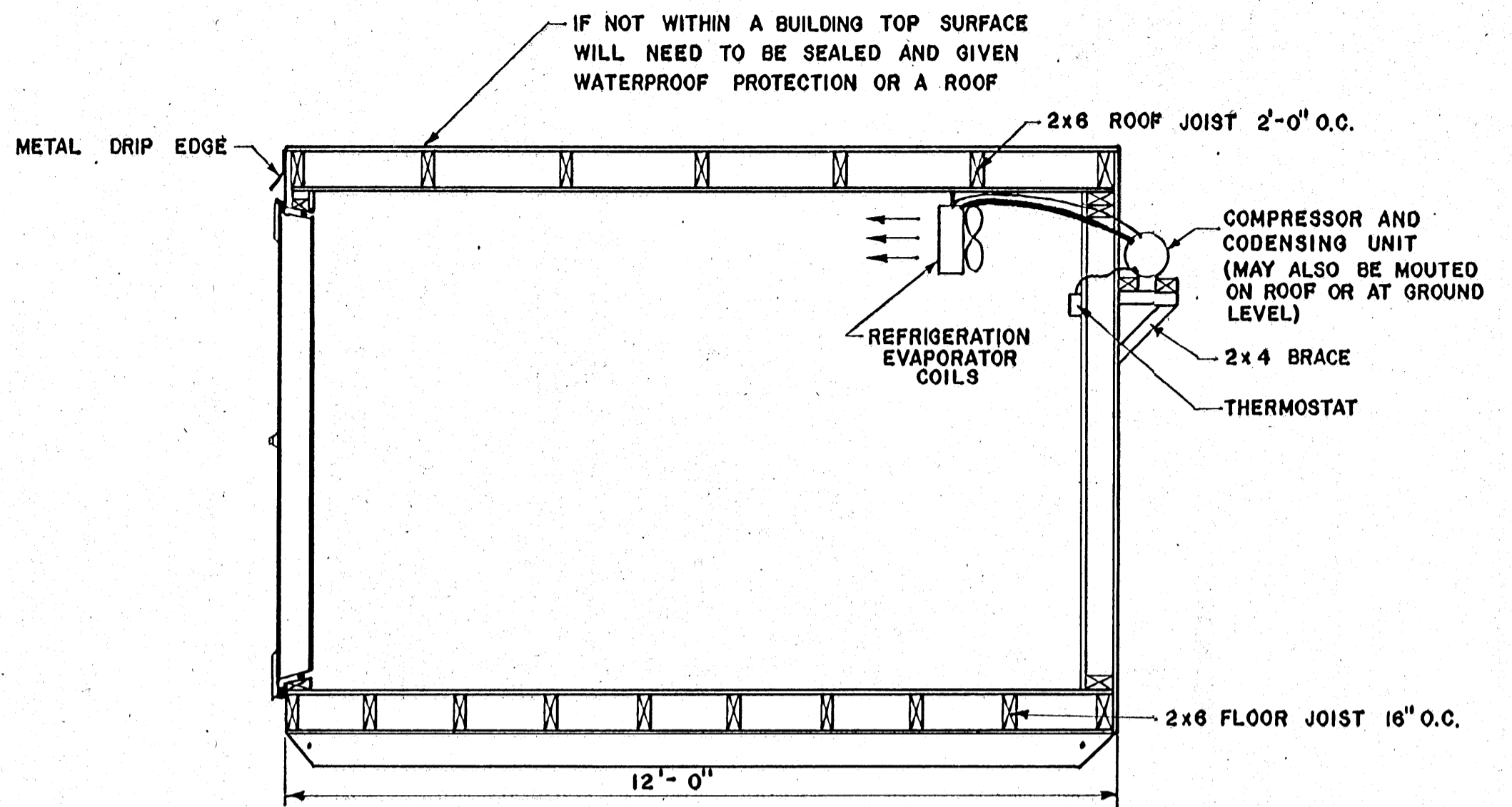
SIDE VIEW
