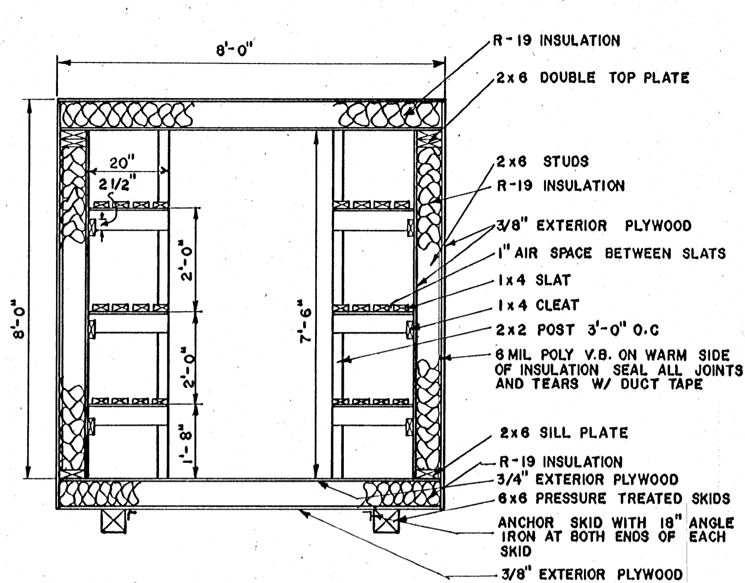
SECTION/SHELF DETAIL
