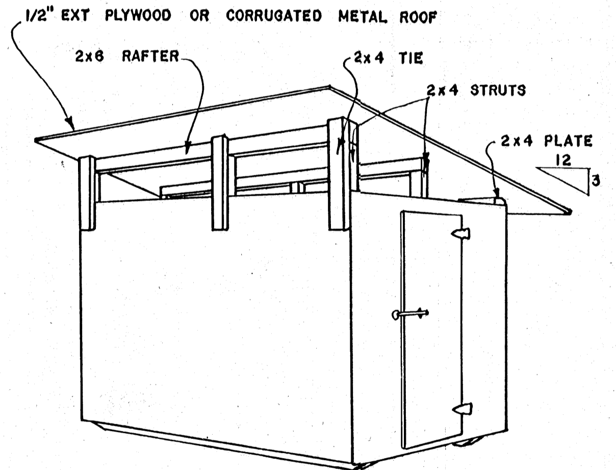
PERSPECTIVE WITH OPTIONAL SHED ROOF (NOT TO SCALE)
