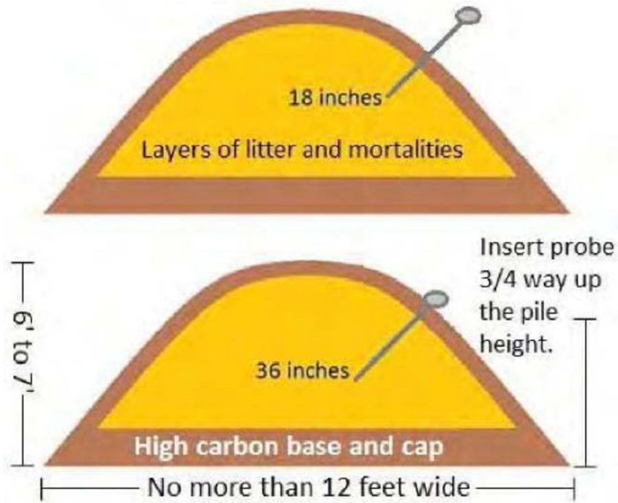
Figure 3. Insert probe thermometer at a 45-degree angle three-fourths of the way up the windrow at 18 and 36 inches.
