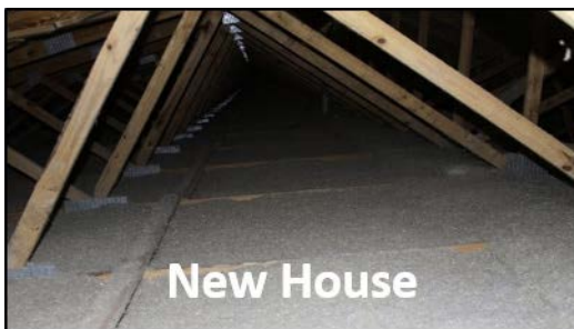
Figure 1. Blown cellulose is filled to the top of the truss’s bottom chord in this new house. In the aging house, the blown cellulose has settled several inches below the top of the bottom chord.
